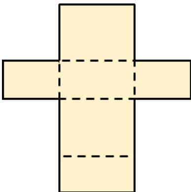
Rectangular Prism
