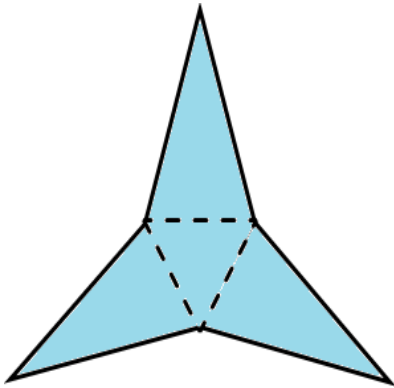
Triangular Pyramid
