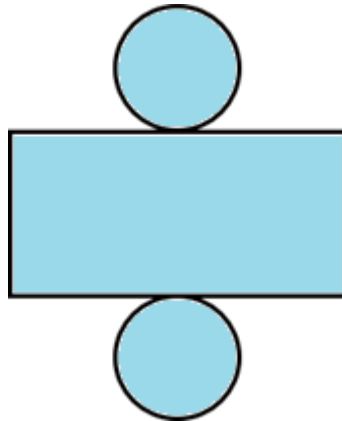
Cylinder
