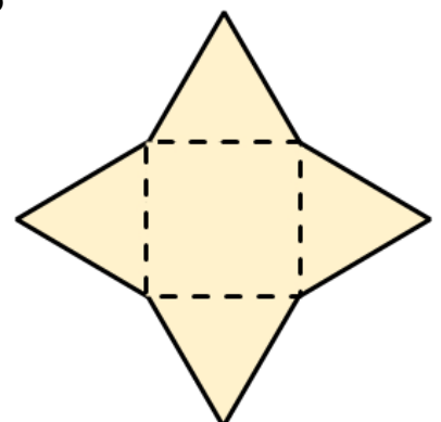
Square Pyramid
