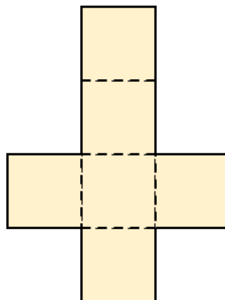
Cube
